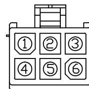
AMP 172168-1 PLUG 170360-1 PIN
