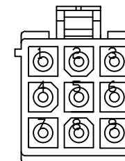
AMP 172169-1 PLUG 170359-1 PIN
