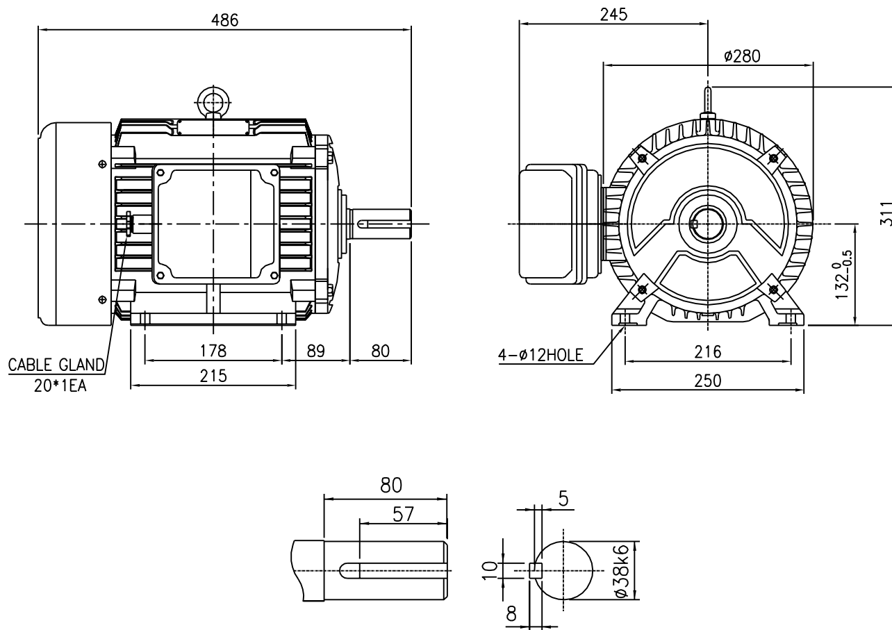
SHAFT EXTENSION
