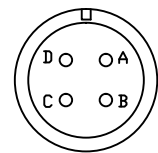
MS3102A22-22P Motor Cable Connector 접속도
