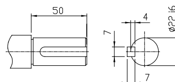
SHAFT EXTENSION
