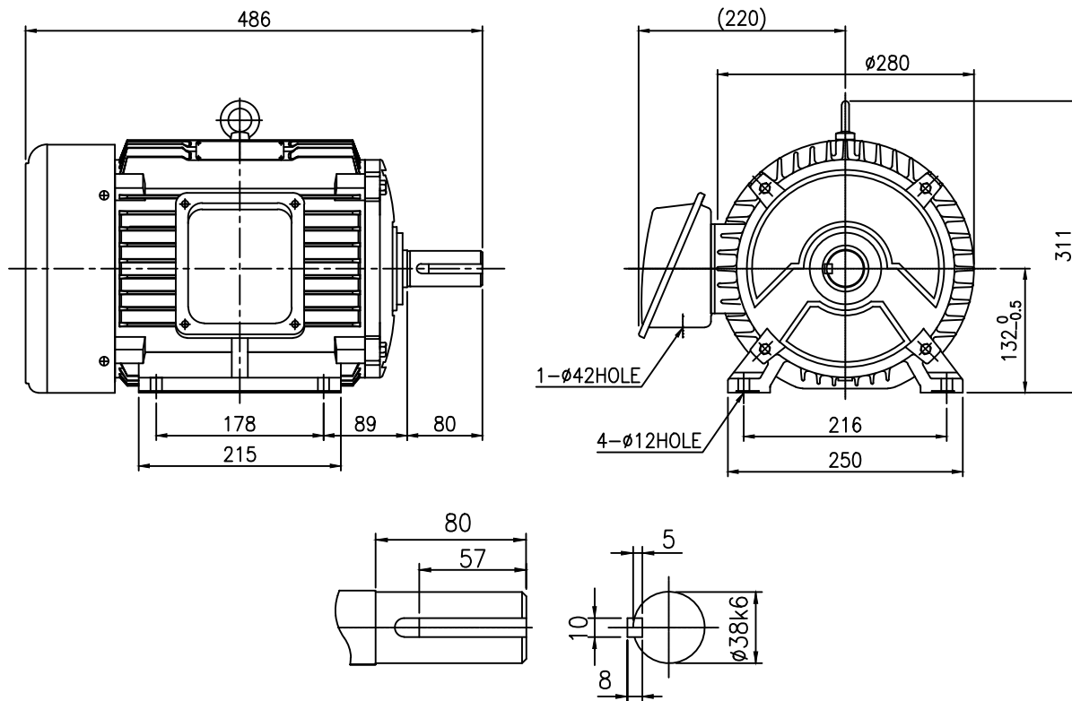
SHAFT EXTENSION
