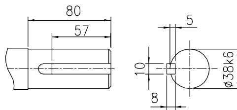
SHAFT EXTENSION
