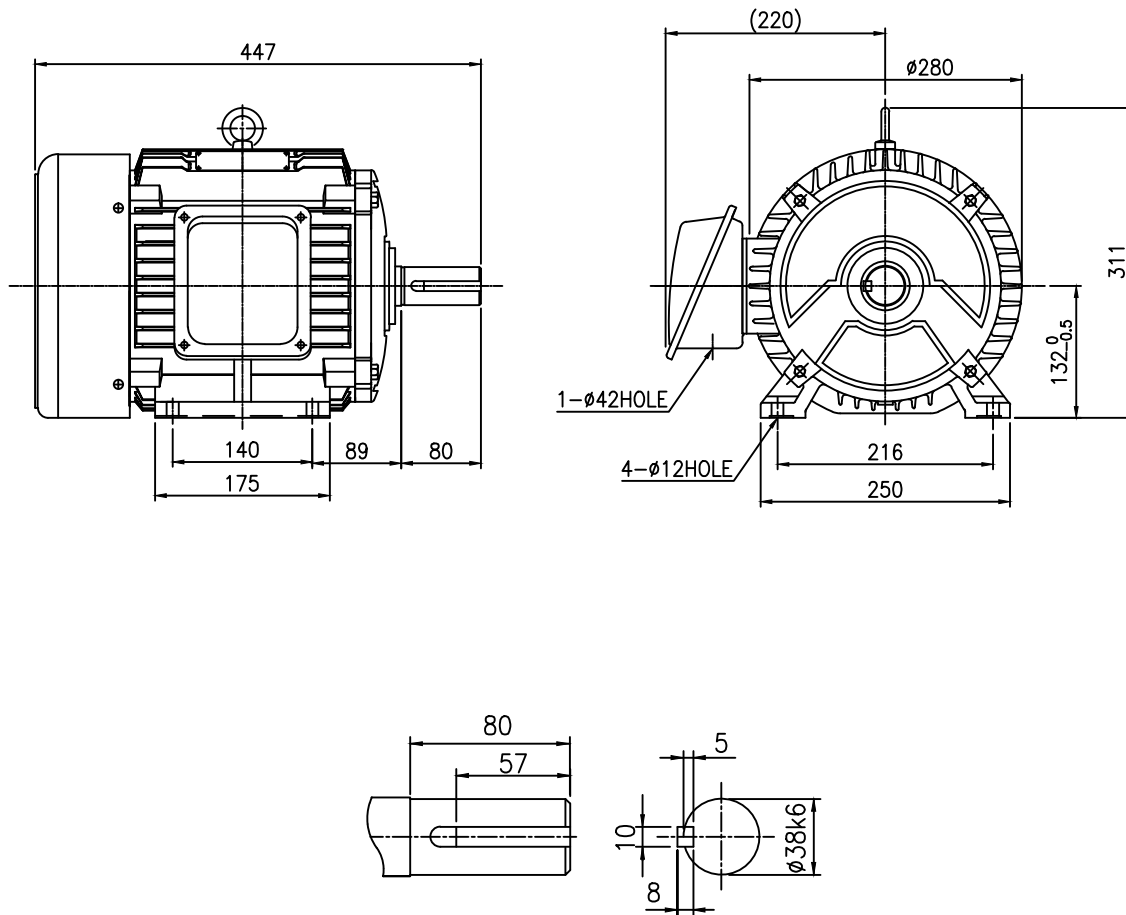
SHAFT EXTENSION
