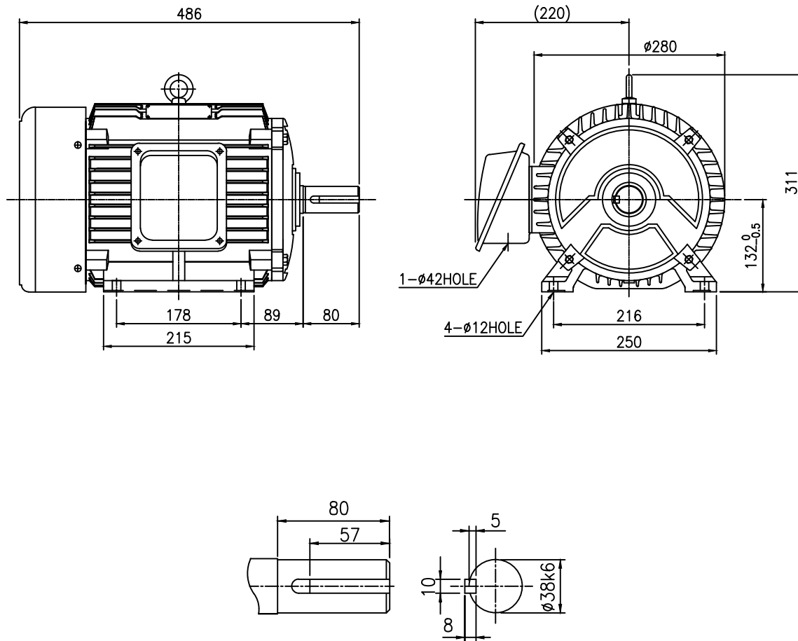
SHAFT EXTENSION
