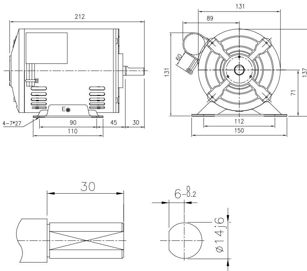
SHAFT EXTENSION
