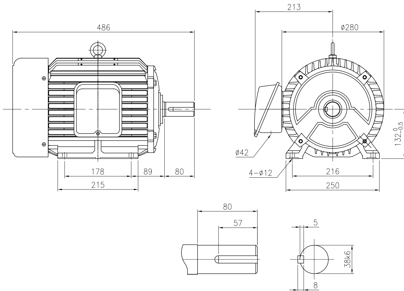
SHAFT EXTENSION
