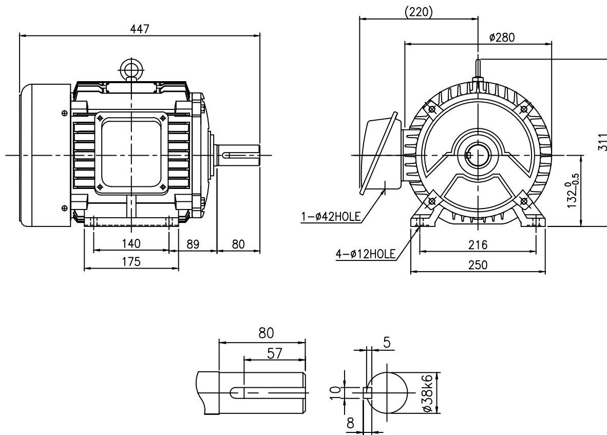
SHAFT EXTENSION
