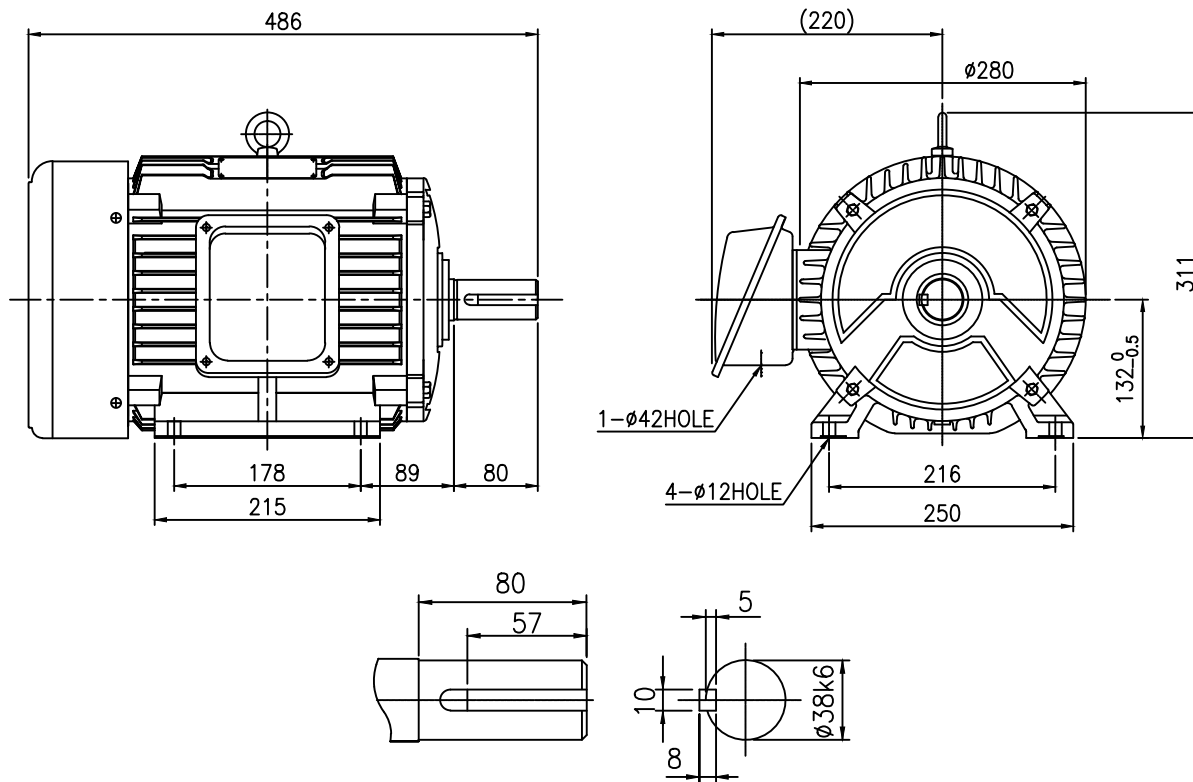
SHAFT EXTENSION
