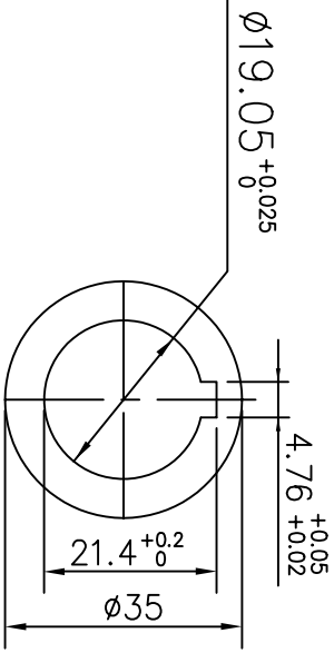
DETAILED OF SHAFT END DRIVE
