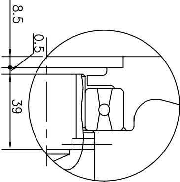
DETAIL OF "Q"
